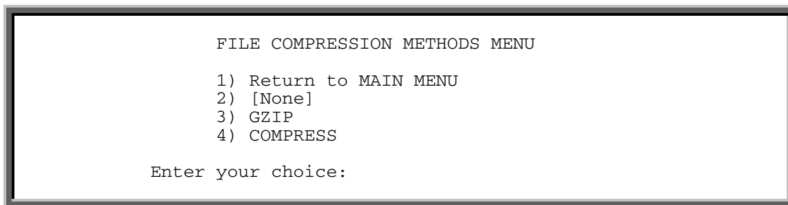
Figure 11. Initial File Compression Methods Menu Display.
