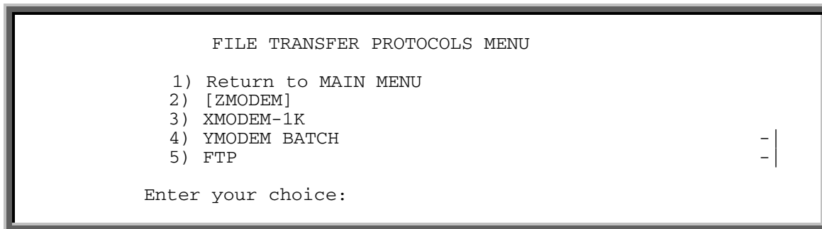
Figure 7. Initial File Transfer Protocol Menu Display
